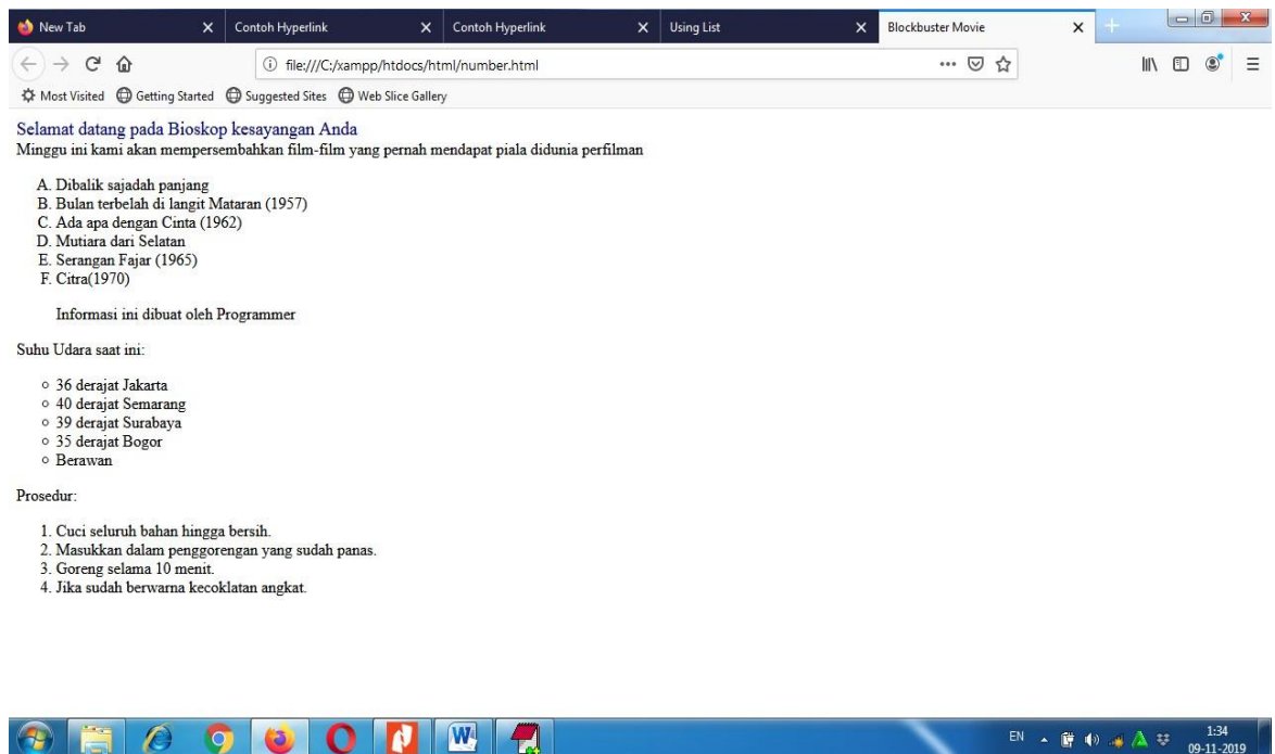
Gambar 19 Tampilan Numbering
