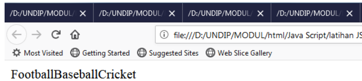
Gambar 70 Output myArray
