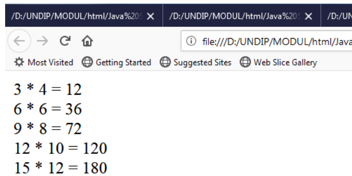
Gambar 59 Tabel perkalian
