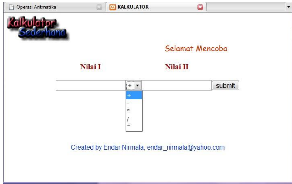
Gambar 55 Tugas Kalkulator
